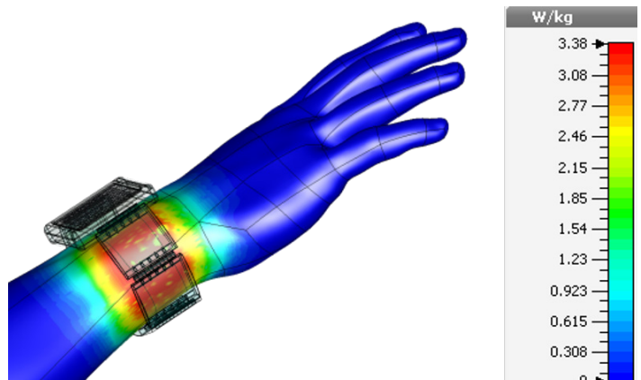
CST calculation EMAG: Antenna radiation Smart watch
