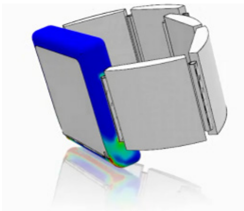
Abaqus calculation of structural mechanics: Drop test Smart watch
